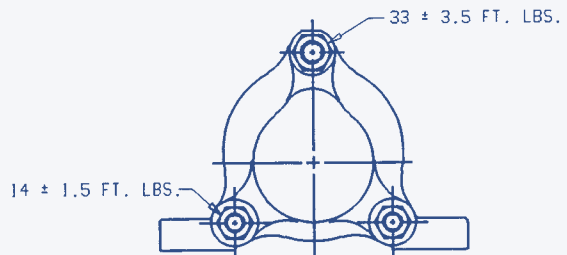
TIE ROD HOLE PATTERN TORQUE - ANY QTY. OF SECTIONS
