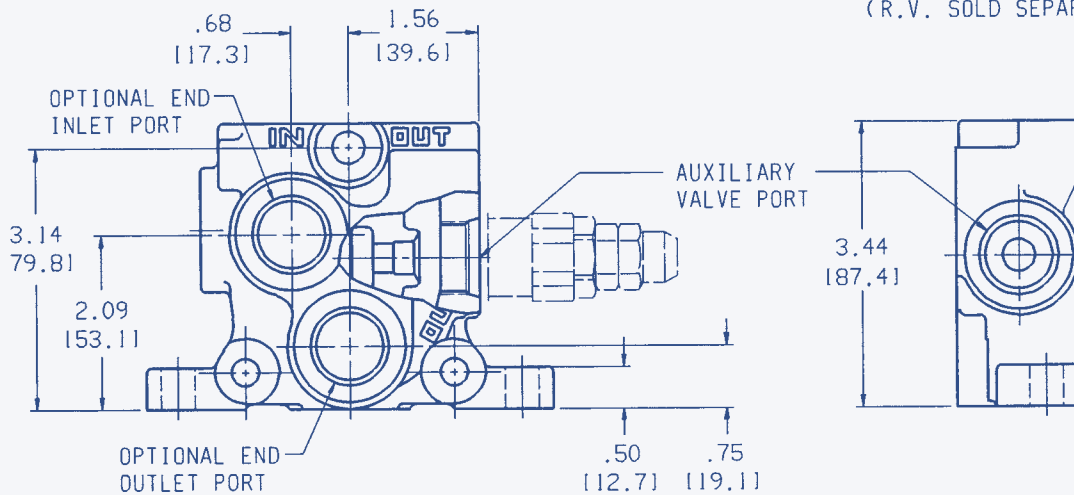
CIRCUIT SHOWN WITH R.V. INSTALLED (R.V. SOLD SEPARATELY)
